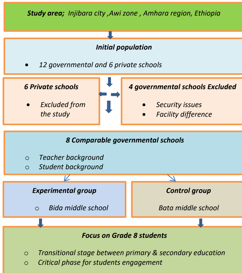
Figure 3 : Sampling procedures
